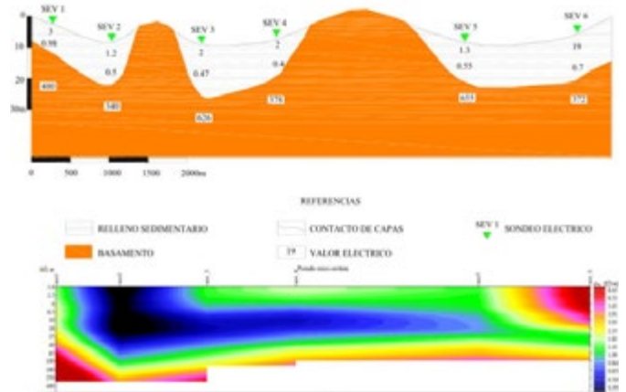
Figure 3: VES Profile – Rincon Salar
