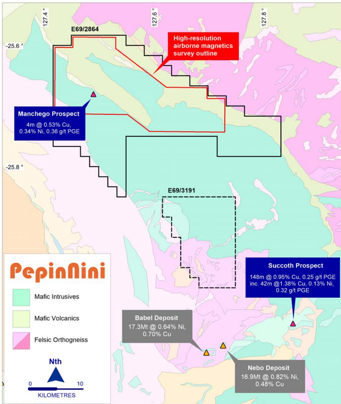
Figure 1: Location of Spinifex Range (E69/2864) airborne magnetics survey with regional geology and Ni-Sulphide occurrences
